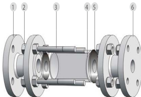
Sight Glass Assembly Detail Drawing
