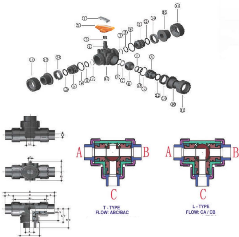
NO. PART MATERIAL Q'TY 1 Cap UPVC/CPVC/PP 1 2 Handle UPVC/CPVC/PP 1 3 O-ring EPDM/ VITON 2 4 Stem UPVC/CPVC/PP 1 5 Seal Carrier UPVC/CPVC/PP 3 6 Ball UPVC/CPVC/PP 1 7 Seat Seal PTFE 4 8 O-ring EPDM/ VITON 4 9 O-ring EPDM/ VITON 3 10 End Connector UPVC/CPVC/PP 3 11 Union Nut UPVC/CPVC/PP 3 12 Body UPVC/CPVC/PP 1 13 O-ring EPDM/ VITON 3 14 Snap ring UPVC/CPVC/PP 3
