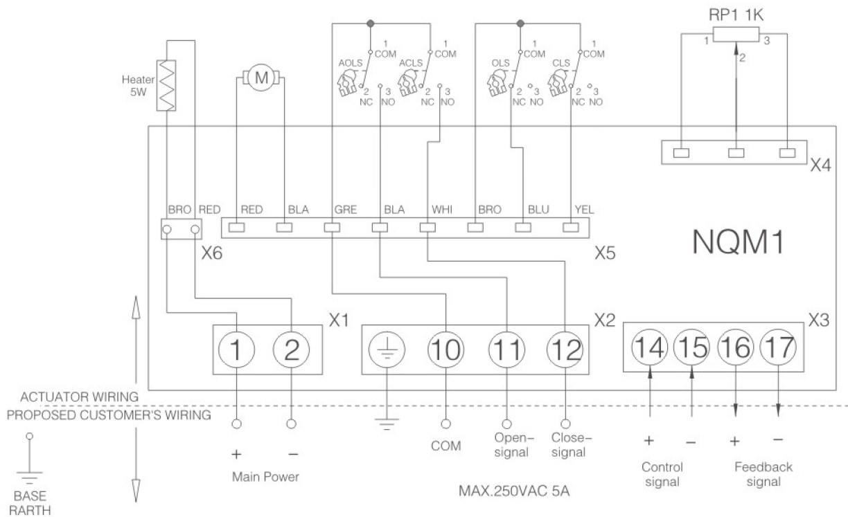
OHVE With Remote Position Controller(24VDC/AC)
