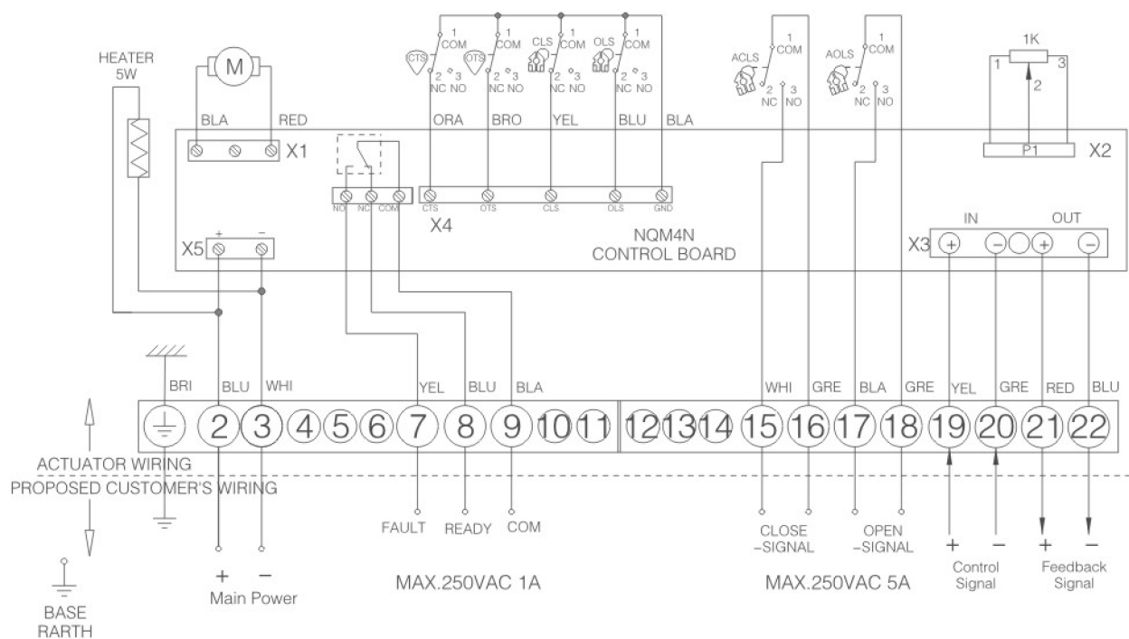
LQ2 With Remote Position Controller(24VDC/AC)
