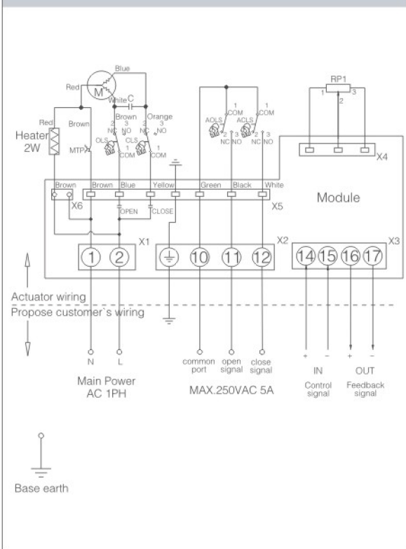
OHVE With Remote Position Controller (1PH AC110V/220V)
